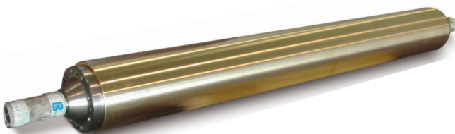
WIPER ROLLERS FOR COLD ROLLING OF ALUMINIUM AND STAINLESS STEEL Material : Aluminium-bronze with high hardness
